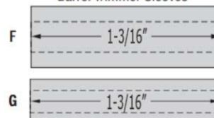
DIAGRAM C • Bushings (#BUFT-7) – Barrel Trimmer Sleeves (#BTS-FT7)
